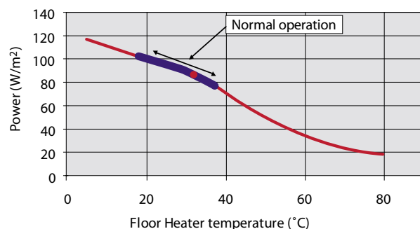
Power characteristics of PTC Under Floor Heating element
